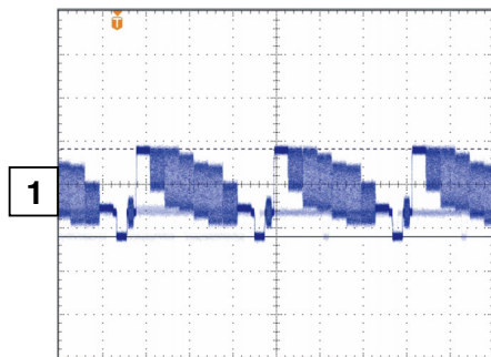
< CVBS_OUT >
